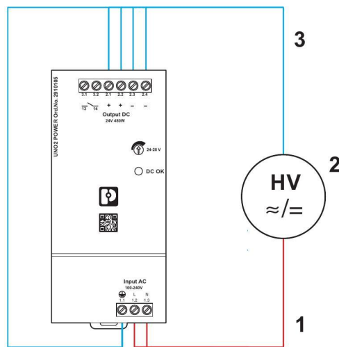
Figure 1 Potential-related wiring for the high-voltage test
