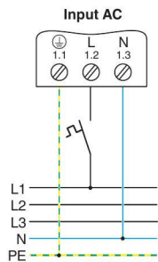
Figure 13 Schematic diagram, single-phase fuse protection
